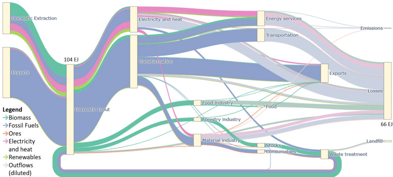
Fig. 2 EU27 resource flows for 2017 based on energy content (1 EJ = 10 18 J). Ores and emissions cannot be meaningfully illustrated in energy flows but are still shown as one-dimensional lines to indicate their relevance based on mass content. Source: own illustration based on refs. [22–24]
